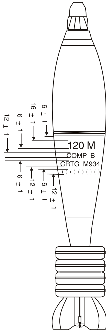
Figure E-75. Typical marking for 120mm Mortar Cartridges M934 and M934A1.
