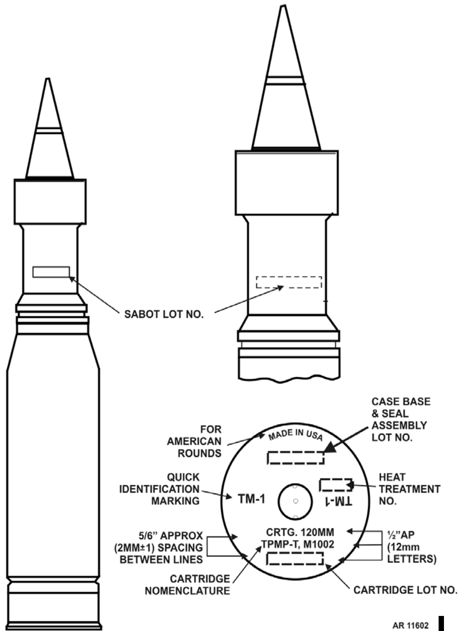
Figure E-71.1. Typical Marking for 120mm Gun Cartridge, TPMP-T, M1002.
